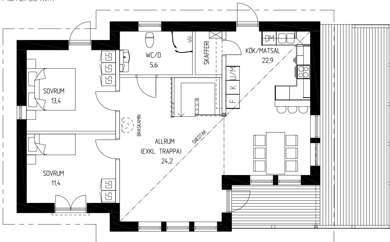
Plan 2: 85 kvm
