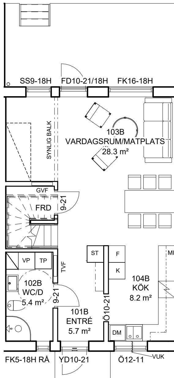
Bottenplan
